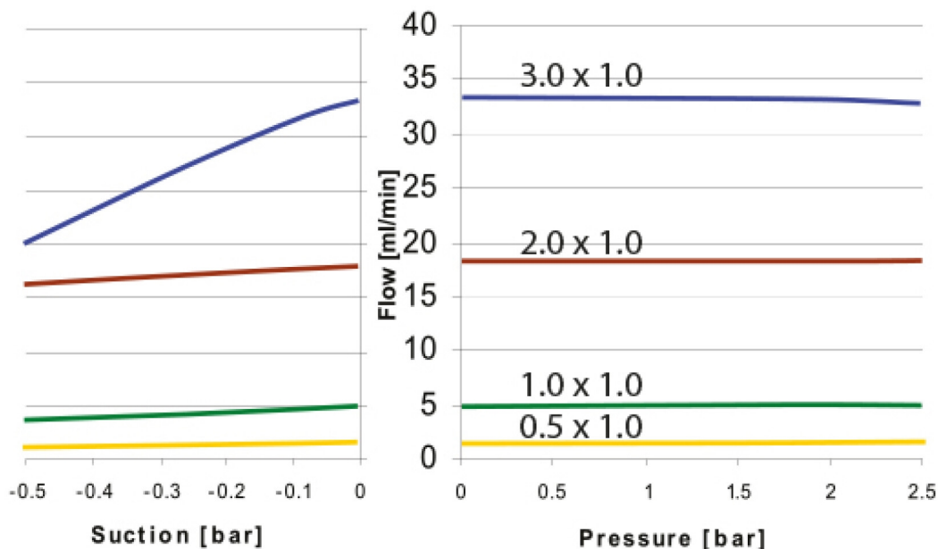
400/N Pressure / suction charts Santoprene tubing @100rpm
