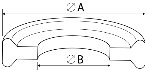
Unflanged type gasket for sizes < 3/4'' flange OD
