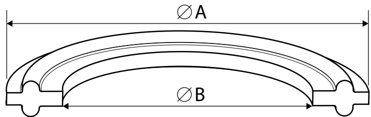
Unflanged type gasket for sizes > 3/4'' flange OD
