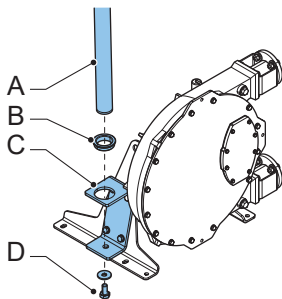
Standardpumpe
